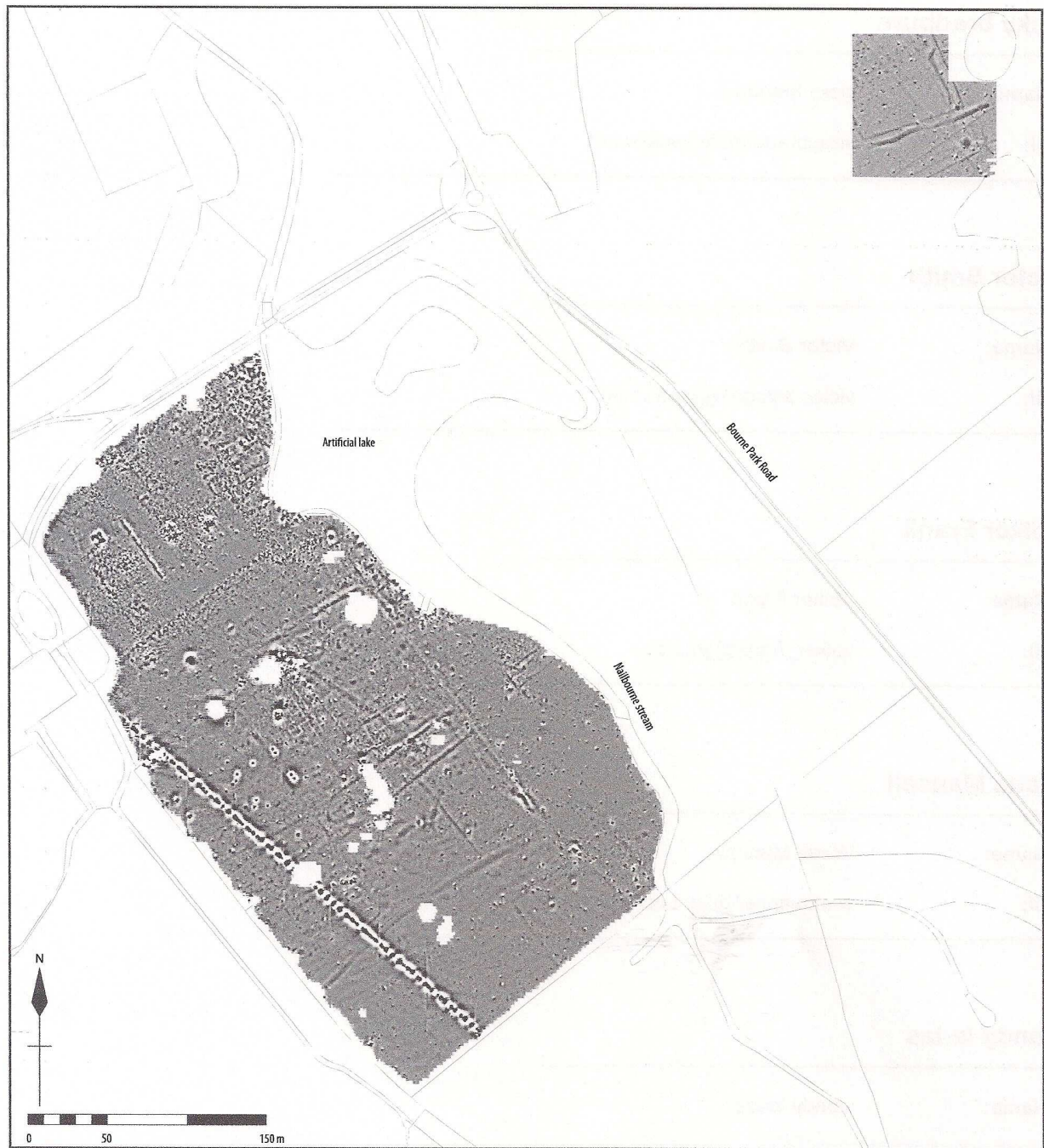
Fig. 12. Processed results of the 2012 gradiometer survey with Ordnance Survey topographical data.
